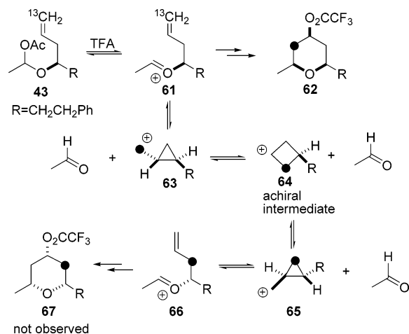
Figure 9. Loss of optical activity for Prins cyclizations is not due to Mechanism C.
