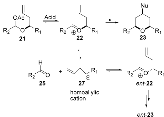
Figure 6. Racemization of Prins cyclization products due to homoallylic cation intermediate (Mechanism D).
