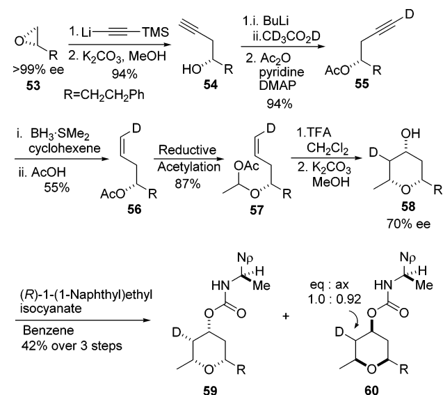
Scheme 3. Synthesis and Prins Cyclization of Deuterated Acetoxy Ether 57
