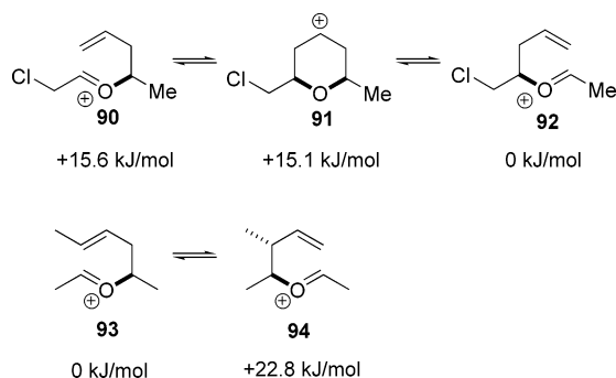
Figure 12. Structural features can reduce the rate of 2-oxonia-Cope rearrangement.
