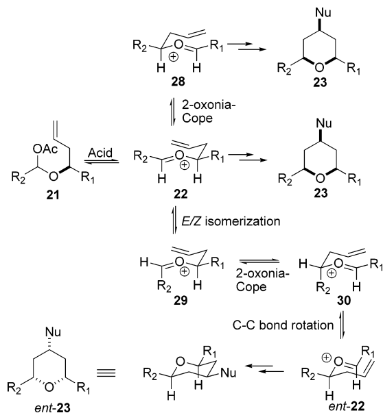
Figure 7. Racemization of Prins cyclization products due to E/Z isomerization and 2-oxonia-Cope rearrangement (Mechanism E).
