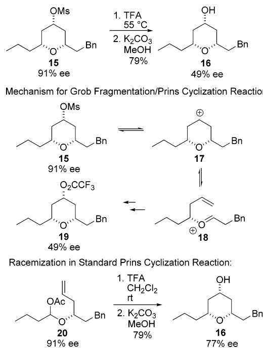
Figure 4. Unusual racemization in Prins cyclizations.
