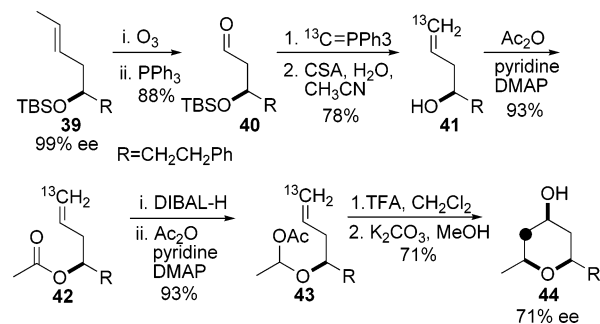
Scheme 1. Synthesis and Prins Cyclization of 13 C-Labeled Acetoxy Ether 43
