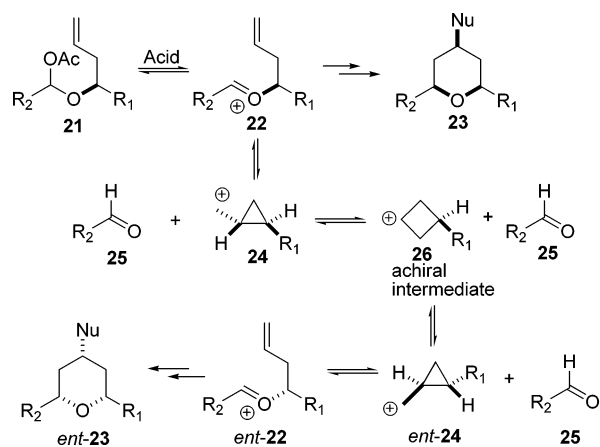
Figure 5. Racemization of Prins cyclization products by achiral cyclobutyl cation intermediate (Mechanism C).
