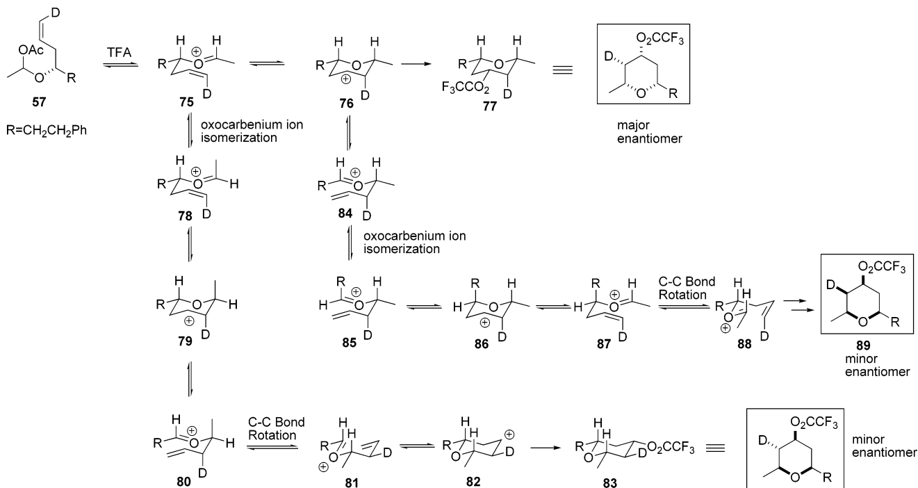
Figure 11. 2-Oxonia-Cope rearrangement through a ( Z )-oxocarbenium ion leads to loss in optical activity for Prins cyclizations.
