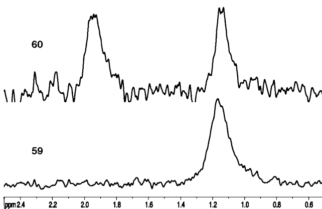
Figure 8. 2 H NMR spectra for tetrahydropyran 59 and tetrahydropyran 60 .
