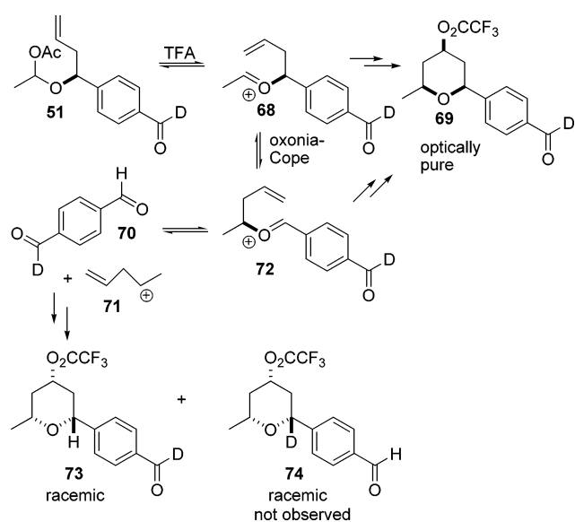
Figure 10. Loss of optical activity for Prins cyclizations is not due to Mechanism D.
