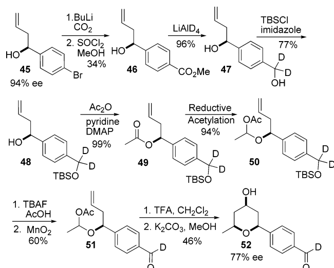
Scheme 2. Synthesis and Prins Cyclization of Deuterated Acetoxy Ether 51
