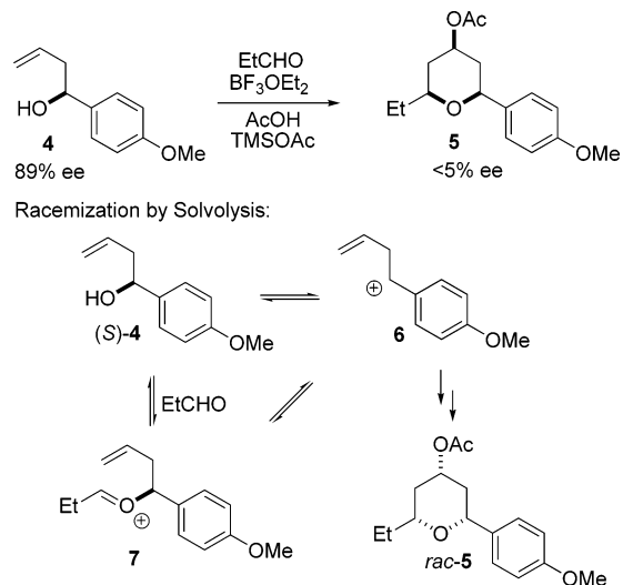
Figure 2. Loss of enantiomeric excess in Prins cyclizations of electron-rich benzylic homoallylic alcohols (Mechanism A).
