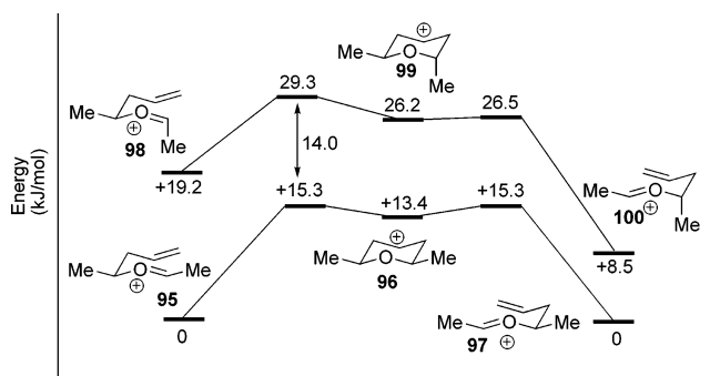
Figure 13. Energetics of enantiomerization.
