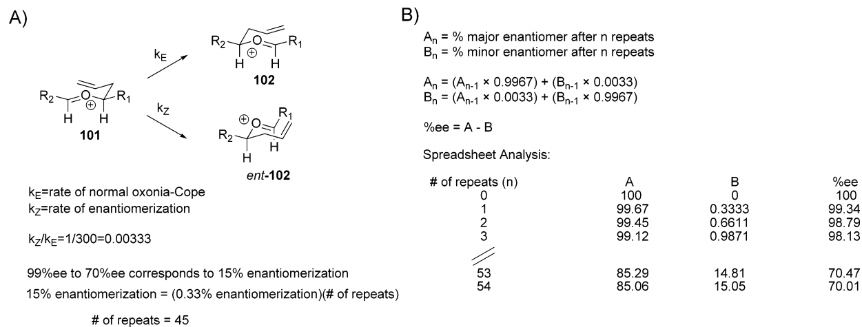
Figure 14. Oxonia-Cope rearrangement must occur many times for a significant loss in optical purity.
