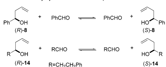
Figure 3. Racemization of Prins cyclization products by symmetric 2-oxonia-Cope rearrangement (Mechanism B).
